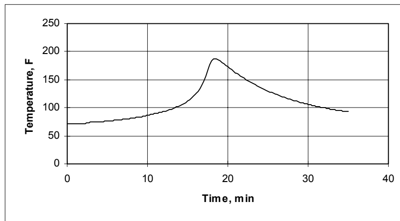
Typical Exotherm Curve for MA3940 at 75°F (10 grams) 5
