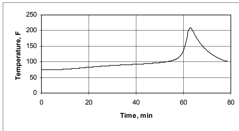
Typical Exotherm Curve for MA925 at 75°F (10 grams) 5
