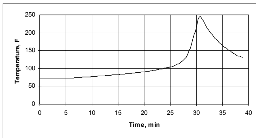
Typical Exotherm Curve for MA922 at 75°F (10 grams) 5
