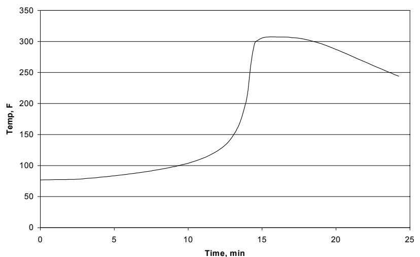
Typical Exotherm Curve for MA821 at 75°F (10 grams) 5
