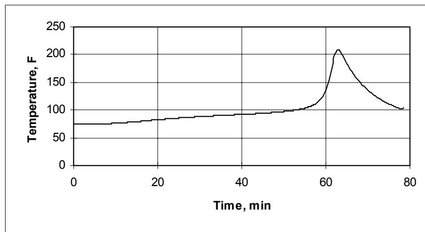
Typical Exotherm Curve for MA425 at 75°F (10 grams) 5
