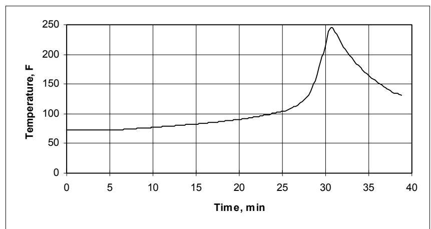
Typical Exotherm Curve for MA422 at 75°F (10 grams) 5
