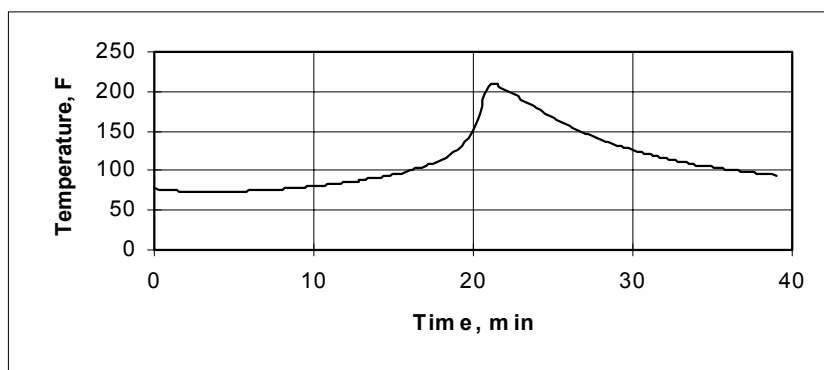
Typical Exotherm Curve for MA320 at 75°F (10 grams) 5
