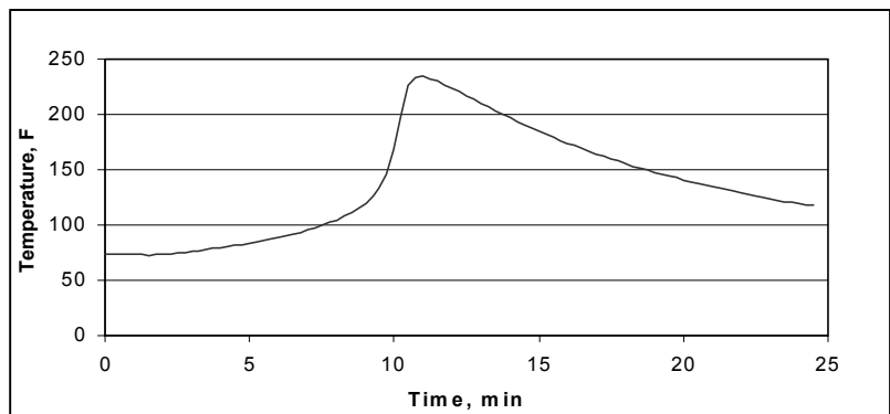
Typical Exotherm Curve for MA1023 at 75°F (10 g.) 5
