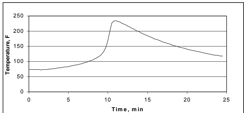
Typical Exotherm Curve for MA1020 at 75°F (10 g.) 5
